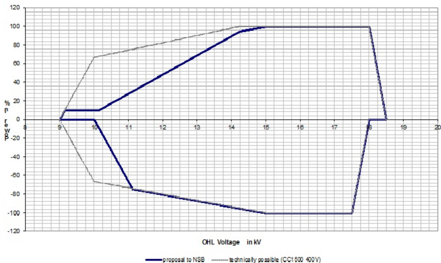
OHL Voltage Dependent Power Reduction
